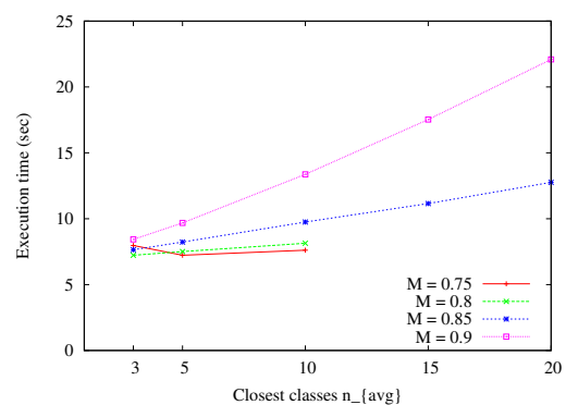
Figure 7: Execution time per recognition vs number of similar views ( n_{avg} ) for recognising 1000 new images against various reduced sets (different values of M ).
