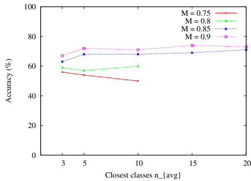
Figure 8: Average accuracy vs number of similar views ( n_{avg} ) for recognising 1000 new images against various reduced sets.
