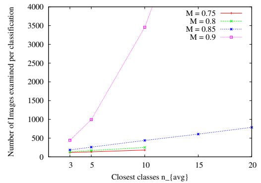
Figure 10: Average number of images examined from each reduced set per classification vs. similar views ( n_{avg} ) for recognising 1000 new images against various reduced sets.
