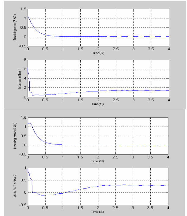
Fig 4.5: The tracking errors and control inputs of the two links when using SMC with the proposed saturated proportional-integral functions in the boundary layers and \alpha = 0.1 ; C_1 = C_2 = 5 , \Phi_1=\Phi_2=0.5 , and K_{I1} = K_{I2} = 75 . Note the errors as e_1=0.000098\text{rad} and e_2=0.00029\text{rad} at t=2\text{s}
