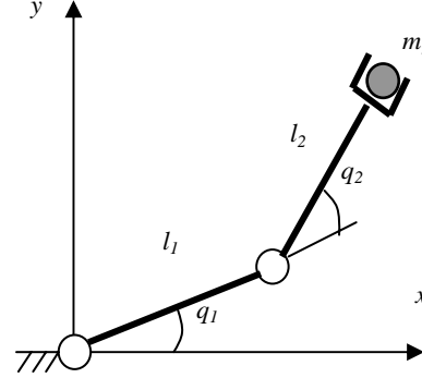
Figure 4.1 : Two-link planar arm
