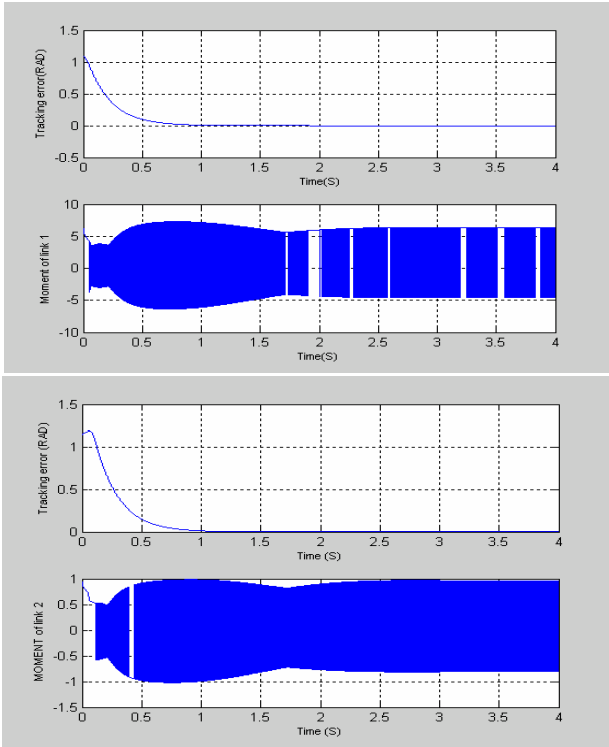
Fig 4.3: The tracking errors and control inputs of the two links under SMC with parameters \alpha = 0.1 , and C_1 = C_2 = 5 . Note the errors as e_1=0.00003\text{rad} and e_2=0.00048\text{rad} at t=2\text{s}
