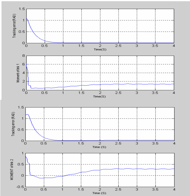
Fig 4.4: The tracing errors and control inputs of 2 links when using conventional SMC with the saturated functions in the boundary layers and \alpha = 0.1 , C_1 = C_2 = 5 , and \Phi_1=\Phi_2=0.5 . Note the errors as e_1=0.00833\text{rad} and e_2=0.0222\text{rad} at t=2.2\text{s}
