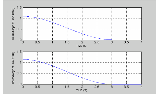
Figure 4.2. The desired time histories of position of two links
